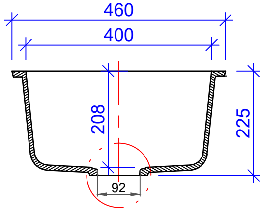
Section view A-A
